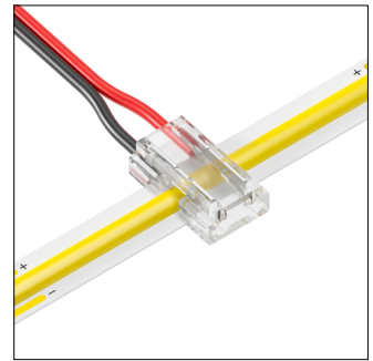
4. Connection completed
