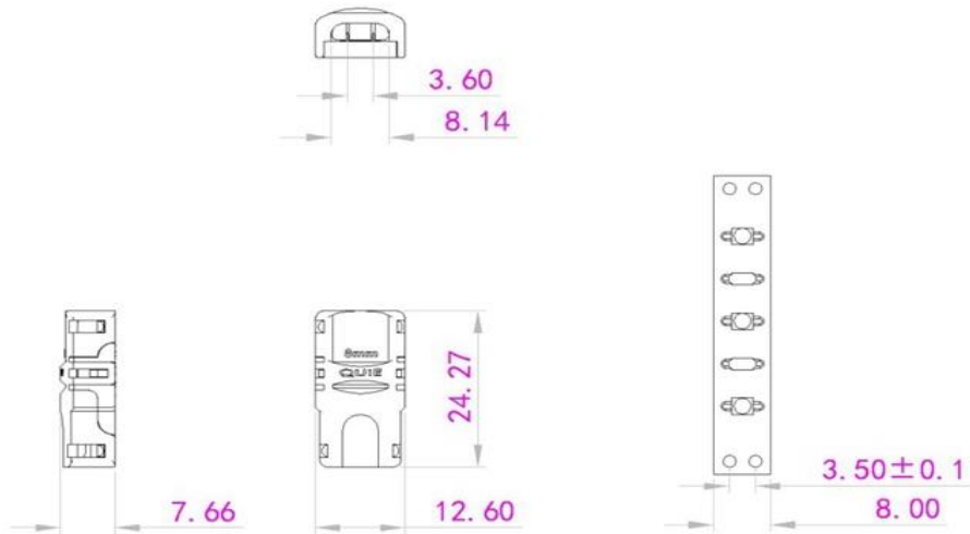
Dimensional Drawing of DJN8XB-2
