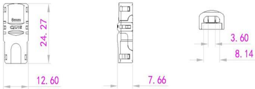
Dimensional Drawing of SEN8XB-2
