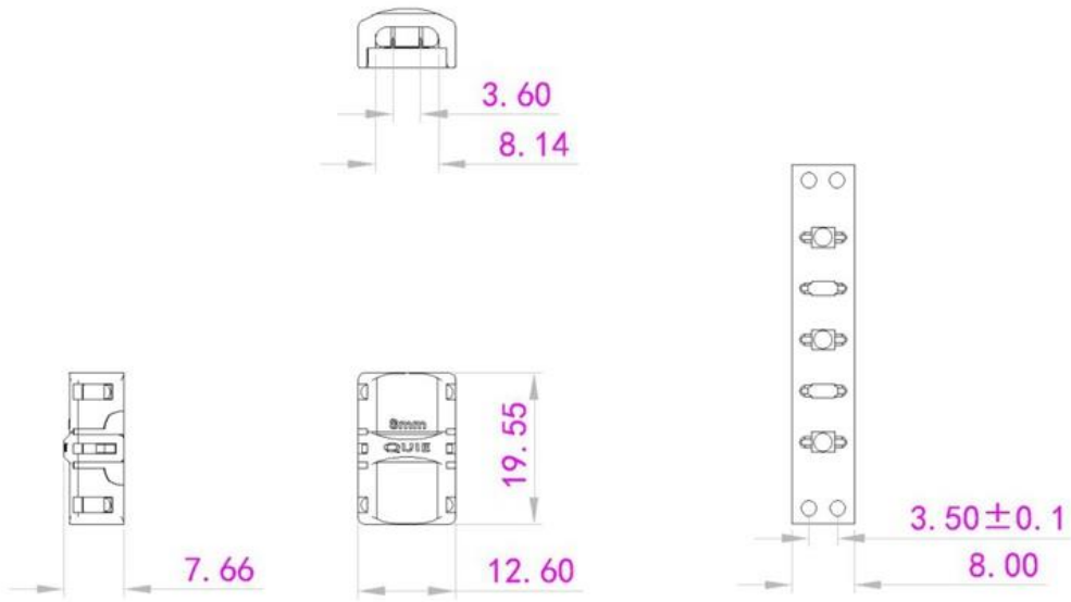
Dimensional Drawing of DJN8BB-2
