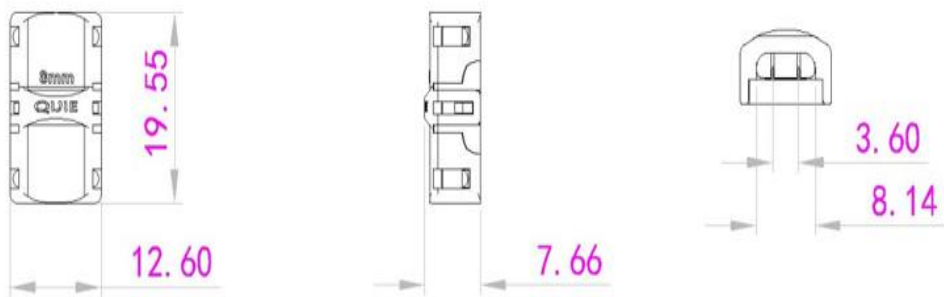
Dimensional Drawing of SEN8BB-2
